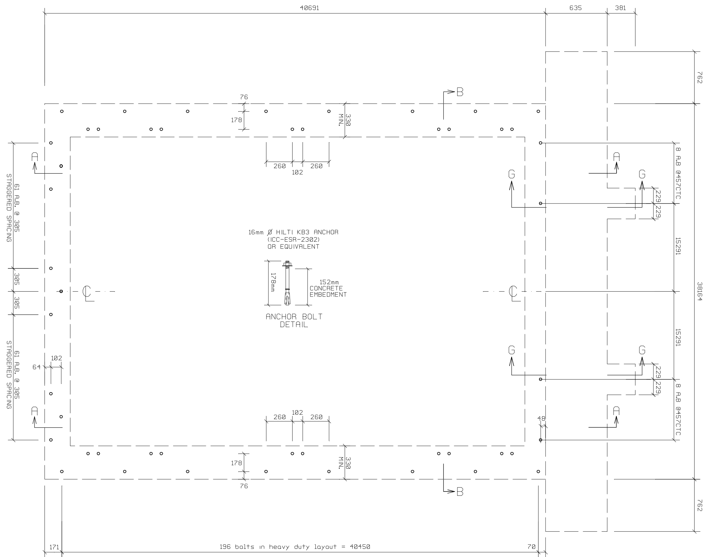
ANCHOR BOLT LAYOUT SUPPORTS/FOUNDATION TO BE DESIGNED BY LOCAL ENGINEER
