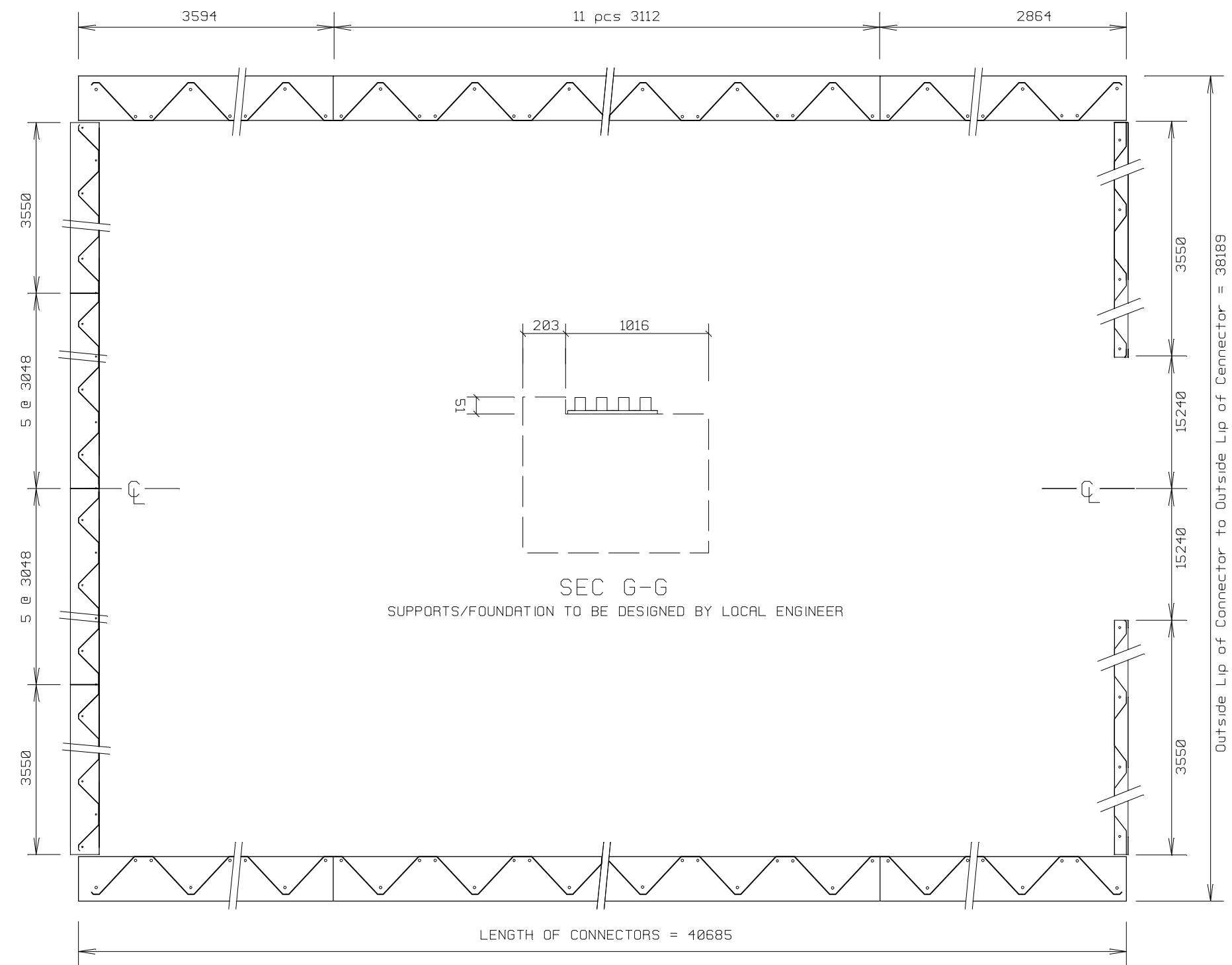
INDUSTRIAL BASE CONNECTOR LAYOUT
